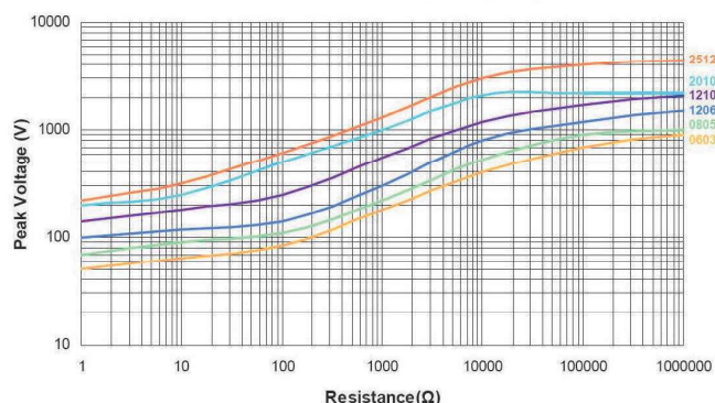
PWR Series 1.2/50us Lightning Surge
