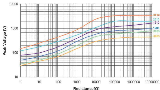
PWR Series 10/700us Lightning Surge
